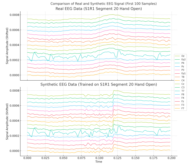
Fig. 6. Comparison of the real EEG signal from segment 20 and the corresponding synthetic signal generated during training. The plot shows the first 100 time points.
